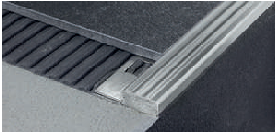
SIS/10 satin stainless steel AISI 304 - DIN 1.4301
