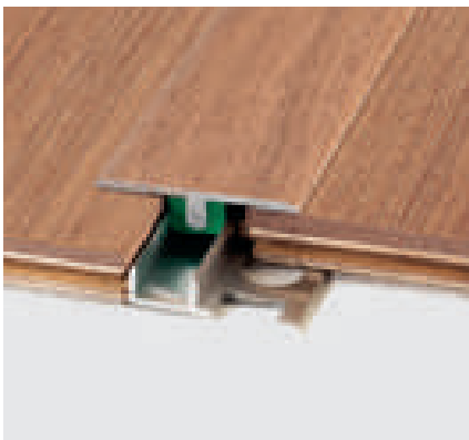
Z/1/SF aluminium covered with Alcrom® Plus film
