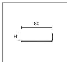
CPLB/2 punched base for tiled floors
