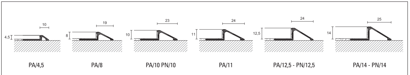
PNI/10 polished stainless steel AISI 304 DIN 1.4301
