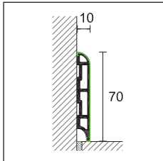
8605 covered with Alcrom® Plus film
