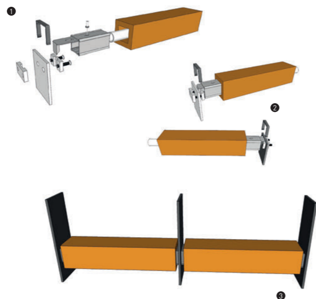
STANDARD SYSTEM
