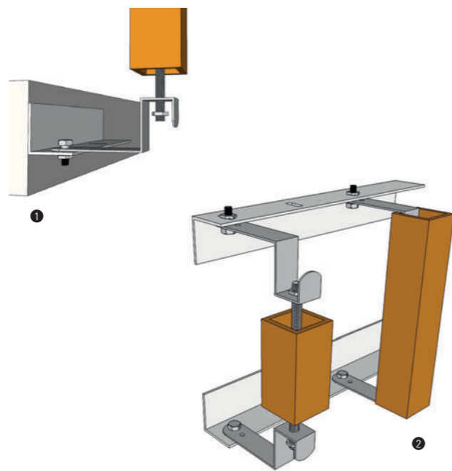
HOOK SYSTEM
