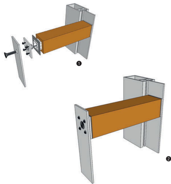
ANCHOR PLATE SYSTEM
